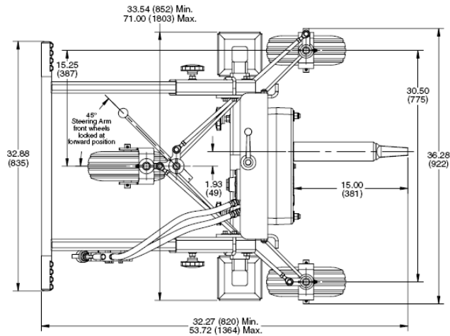
DIMENSIONS—in. (mm)
